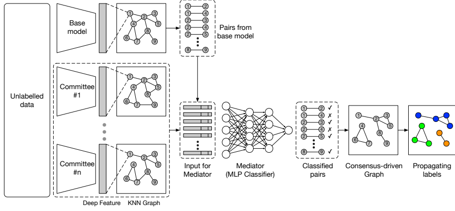
Fig. 1: Consensus-Driven Propagation. We use a base model and committee models to extract features from unlabelled data and create k-NN graphs. The input to the mediator is constructed by various local statistics of the k-NN graphs of the base model and committee. Pairs that are selected by the mediator compose the “consensus-driven graph”. Finally, we propagate labels in the graph, and the propagation for each category ends by recursively eliminating low-confidence edges.
